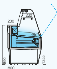
VPRTRV - VC vitrina serve-over counter 3M2 (-1... +7 °C) DIM. 980 | 1280 | 1480 1880 | 2480
