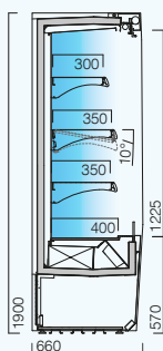
MPRT mural multideck 3M1 (-1... +5 °C) DIM. 680 | 980 | 1280 1480 | 1880
